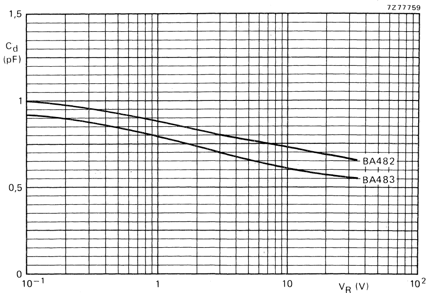
Fig. 4 Typical values; f = 1 to 100\text{ MHz} ; T_j = 25^\circ\text{C} .
