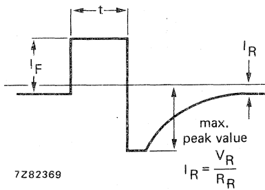
Fig. 3 Output waveform.
