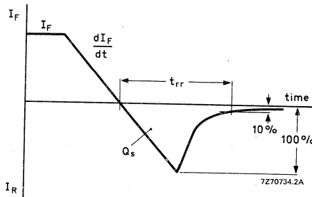
Fig. 6 Definitions of t_{rr} and Q_s .
