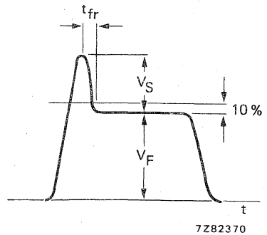
Fig. 4 Waveform.
