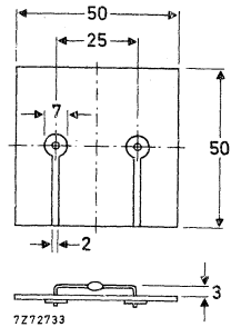
Fig. 4 Mounting method 3.
