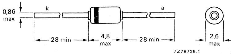
Fig. 1 DO-41 (SOD-66).
