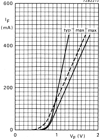
Fig. 12 Forward current as a function forward voltage. — T_j = 25 °C; - - - T_j = 175 °C.
