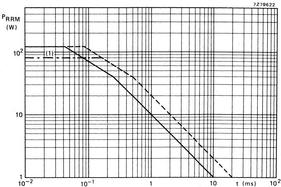
Fig. 10 Maximum permissible repetitive peak reverse power as a function of pulse duration. T > 50 \text{ ms} ; T_j = 25 \text{ }^\circ\text{C} .
