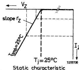
Fig. 5 Static characteristics.
