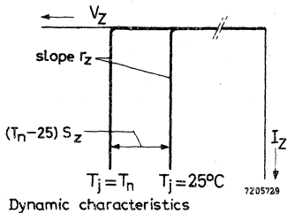
Fig. 4 Dynamic characteristics.
