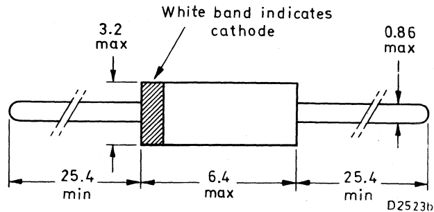
Fig.1 DO-15 The diodes are type branded.
