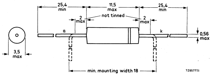
SOD-34 (medium leads) BY409A
