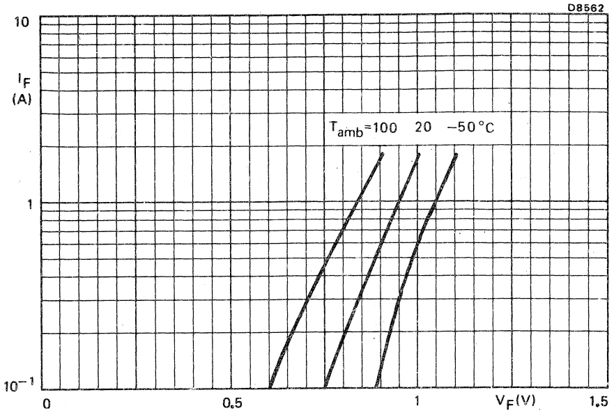
Fig.3 Typical values
