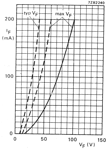
Fig. 6 — T_j = 25^\circ\text{C} ; --- T_j = 120^\circ\text{C} .
