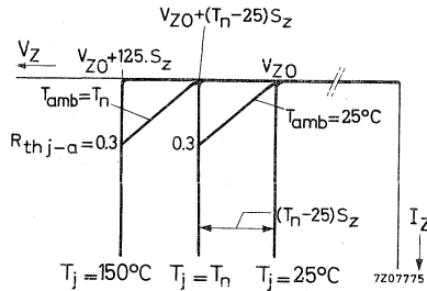
Fig. 7 Example for positive S_z .
