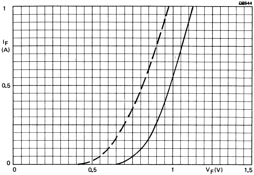
Fig.10 Typical values; — T_j = 25\text{ }^\circ\text{C} ; - - - T_j = 150\text{ }^\circ\text{C}
