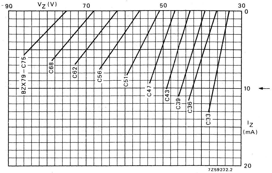
Fig. 10 Static characteristics; typical values; T_{amb} = 25^\circ C .
