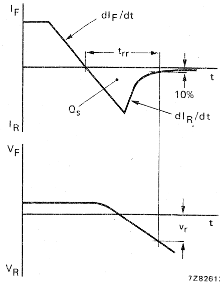
Fig. 4 Definitions.
