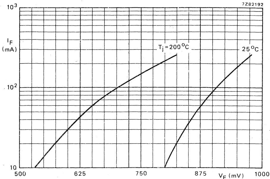
Fig. 12 Typical values.
