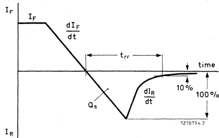
Fig. 3 Definitions of Q_s , t_{rr} and dI_R/dt .
