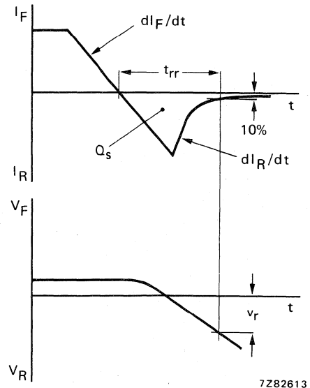
Fig. 4 Definitions.
