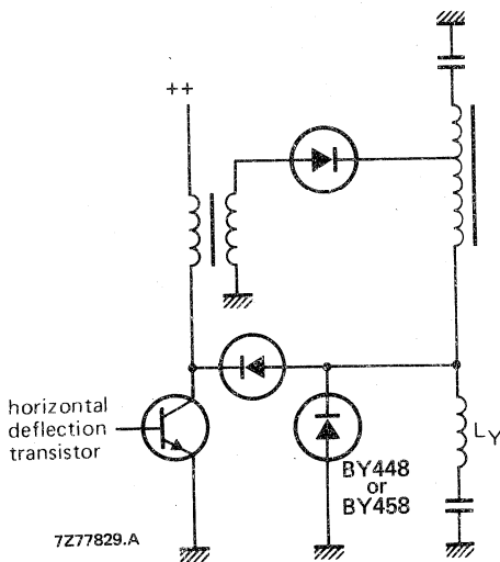
Fig. 10 Basic self-regulating time base circuit (S.R.T.).
